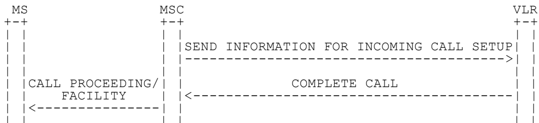
Figure 5.9: Signalling flow for notification of CUG invocation to served MS
