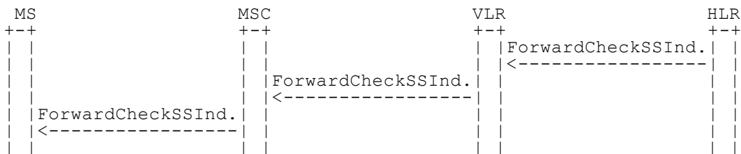
Figure 6.8: ForwardCheckSSIndication
