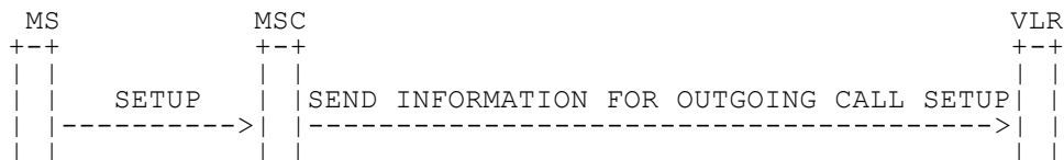
Figure 5.8: Signalling at explicit invocation of a CUG call
