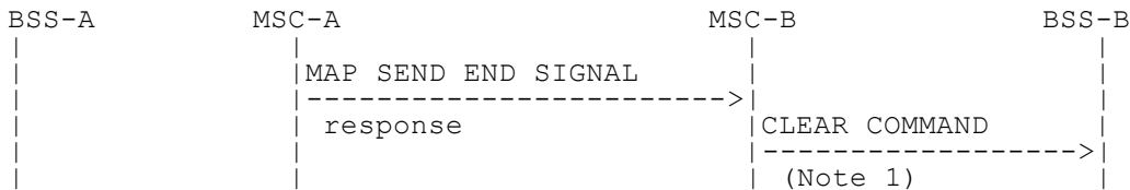
Figure 9: Signalling for Basic Inter-MSC Handover completion (Positive outcome)
