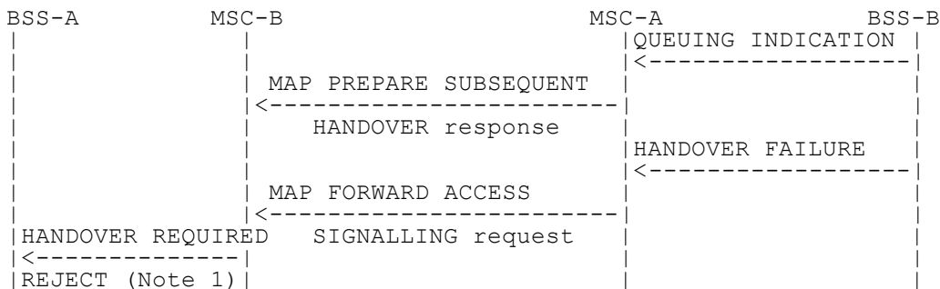
Figure 13: Signalling for Subsequent Inter-MSC Handover back to MSC-A execution (Negative outcome)
