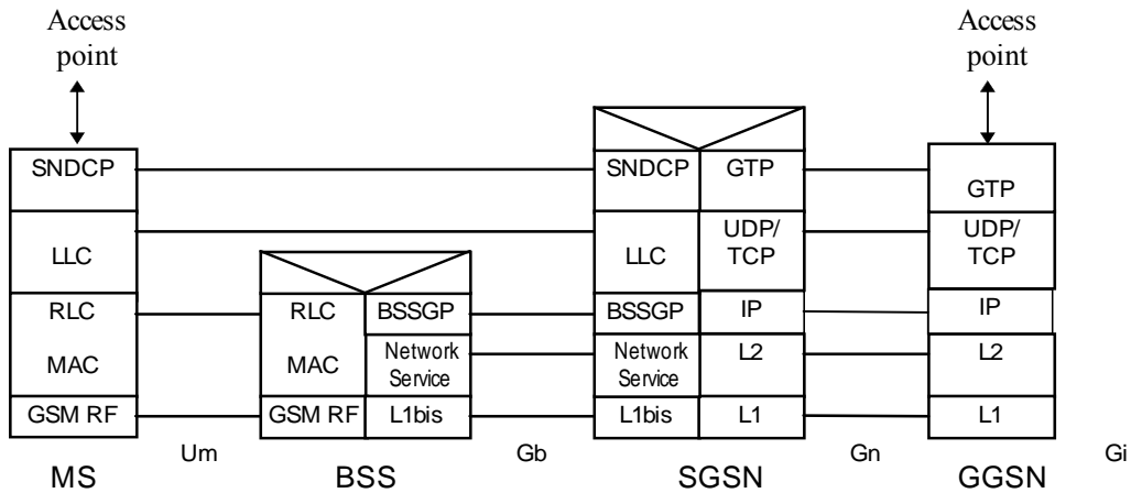
Figure 2: GPRS Transmission Plane
