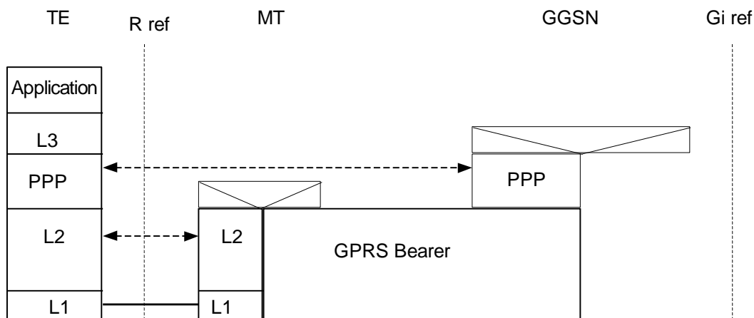
Figure 8: PPP Based Services
