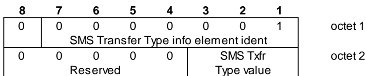
Figure 2.5.3/GSM 07.05: SMS Transfer Type information element
