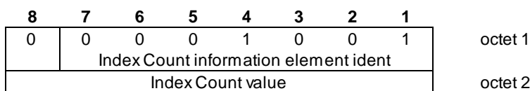
Figure 2.5.11/GSM 07.05: Index Count information element
