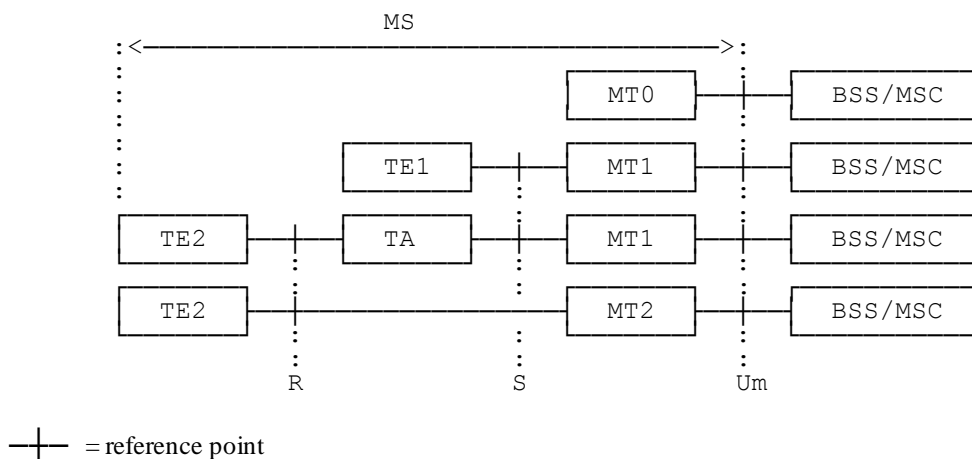
Figure 1 presents the reference configuration for access to a GSM PLMN (see GSM 04.02).
