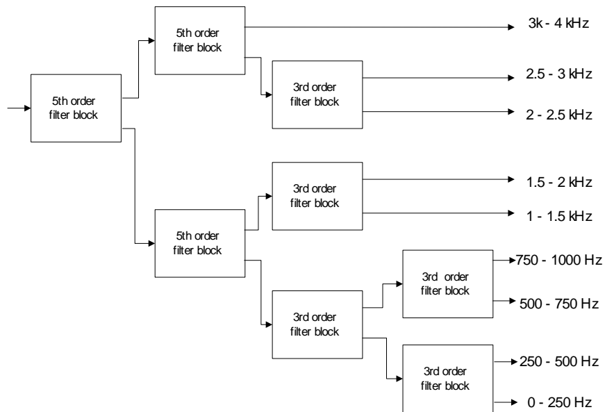
Figure 3.2: Filter bank
