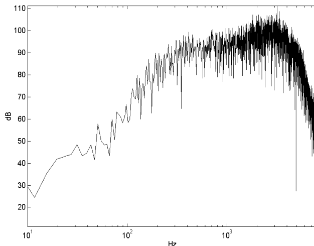
Figure 3: Frequency response of the M-IRS filtering module
