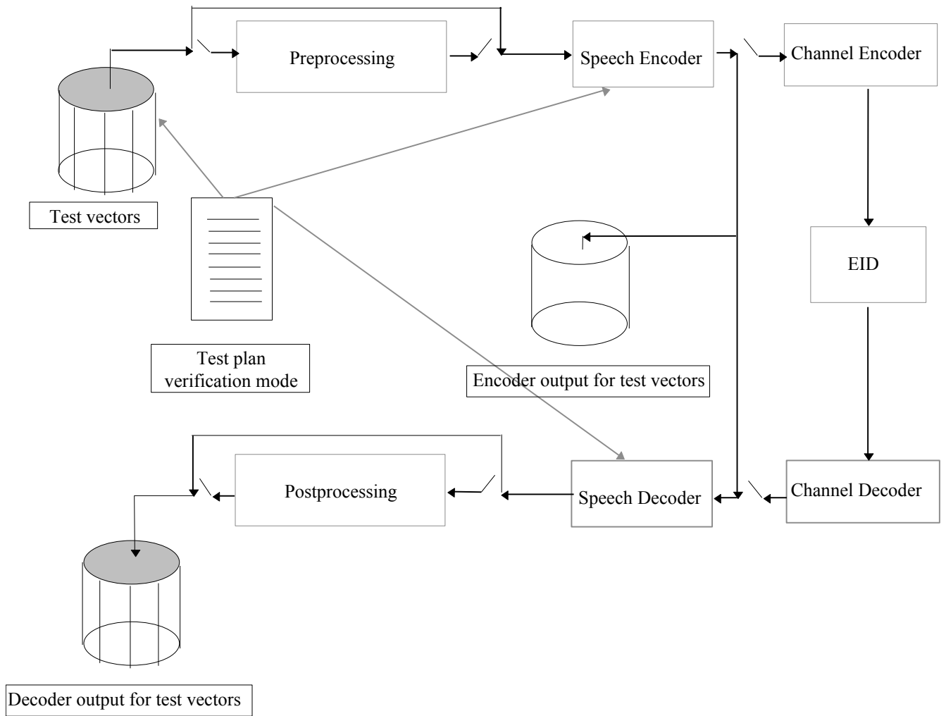
Figure 2: Scheme of the testing procedure using the test vectors
