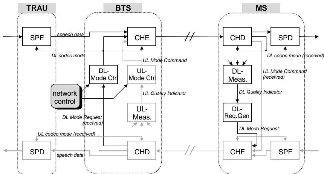
Figure 2: Block diagram of the AMR system.
