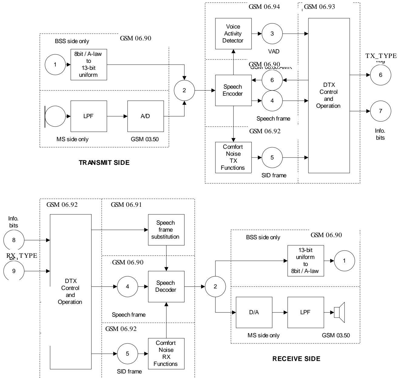
Figure 1: Overview of audio processing functions
