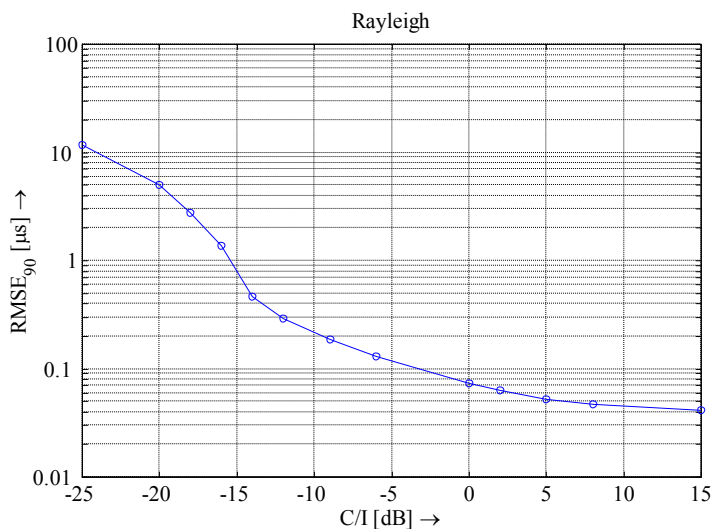
Figure V.4.7. TOA estimation error (in \mu s) as function of C/I in a flat Rayleigh fading channel.
