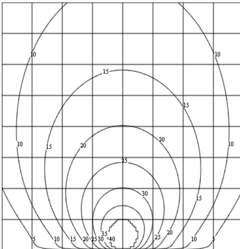
Figure X.7 Geometric C/I contours for N=4/12 reuse pattern.
