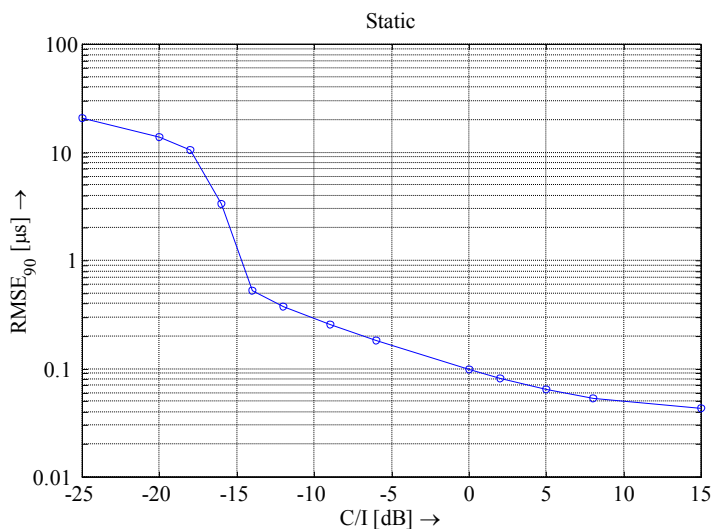
Figure V.4.6. TOA estimation error (in \mu s) as function of C/I in a static channel.
