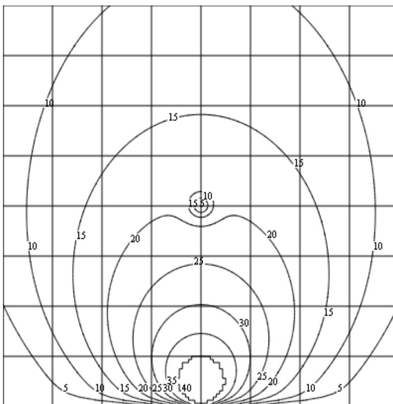
Figure X.11 Geometric C/I contours for worst-case interfering cell (interferer at -60 dBc).
