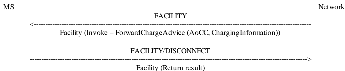
Figure 2.3: Notification to the served mobile subscriber of a change in the charging information
