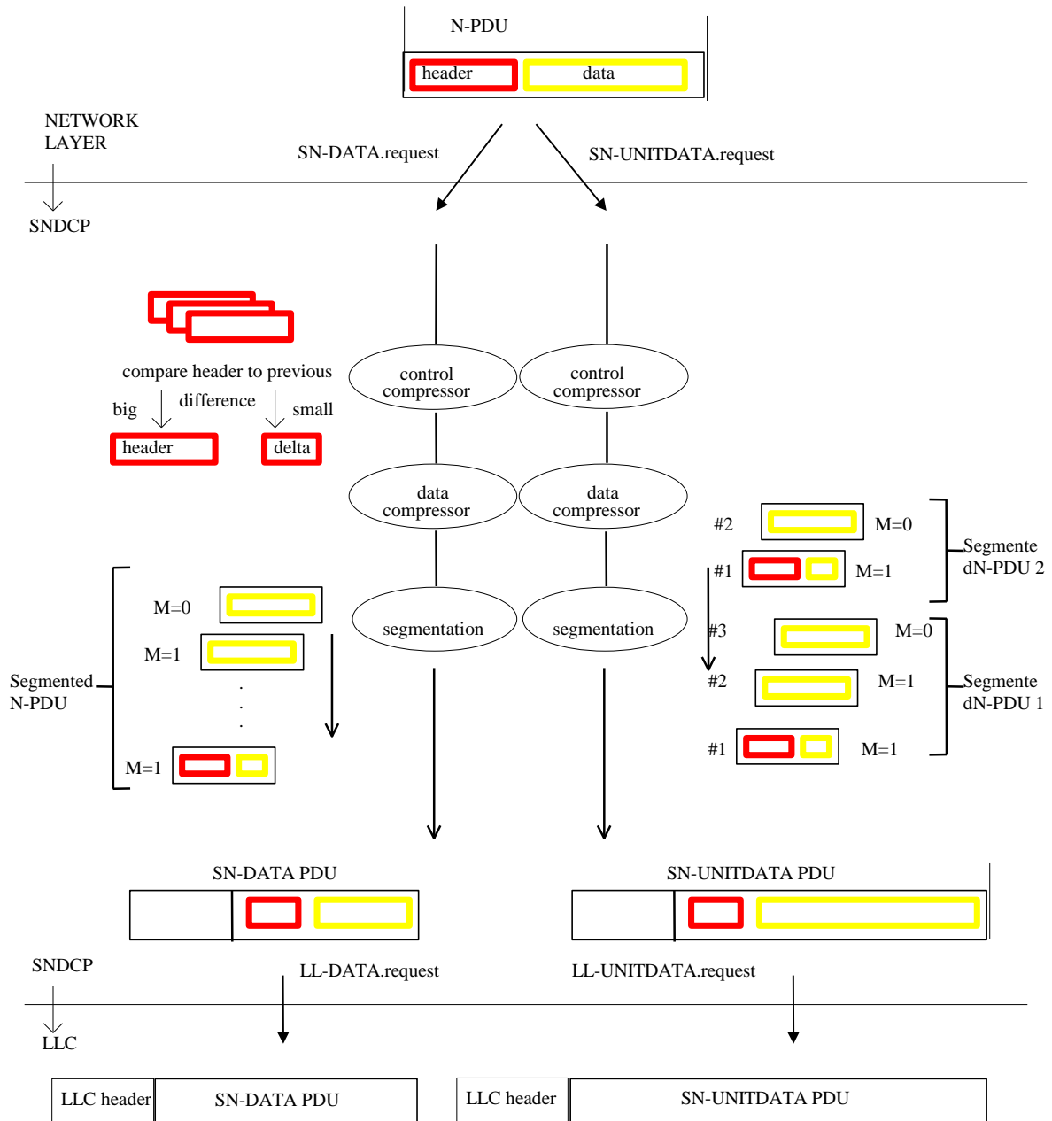
Figure 4: SNDCP model
