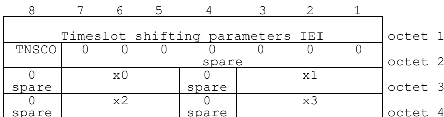
Figure 10.24/GSM 04.56 Timeslot shifting parameters information element
