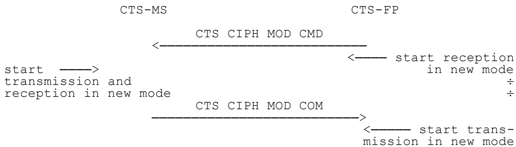
Figure 4.6/GSM 04.56: Cipherng mode setting sequence
