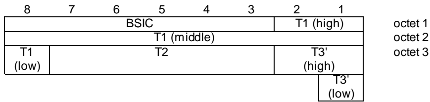
Figure 9.3a/GSM 04.18: Frame synchronization information element
