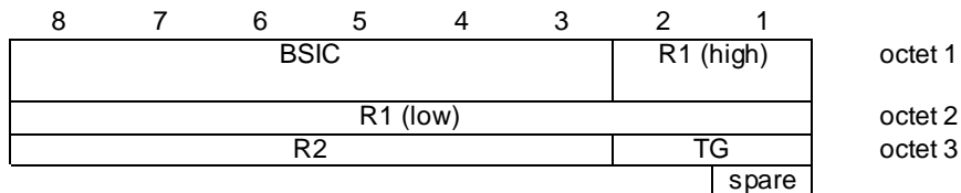
Figure 9.3b/GSM 04.18: COMPACT Frame synchronization information element
