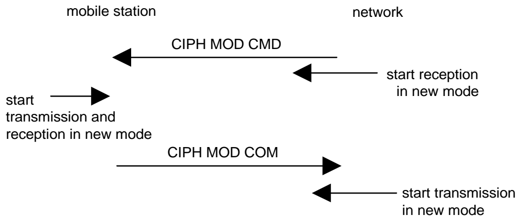
Figure 3.3/GSM 04.18: Ciphering mode setting sequence
