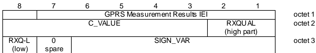
Figure 10.5.48/GSM 04.18 GPRS Measurement Results information element
