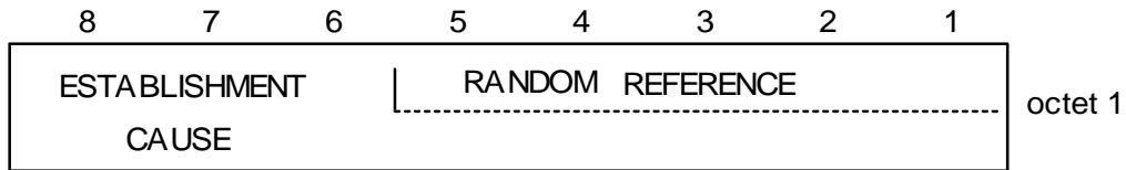
Figure 9.4/GSM 04.18 UPLINK ACCESS message content
