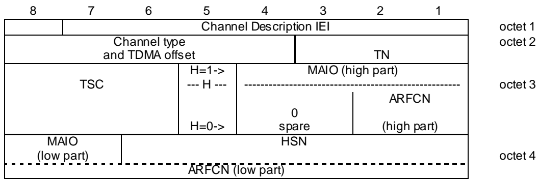
Figure 10.5.26/GSM 04.18 Channel Description 2 information element
