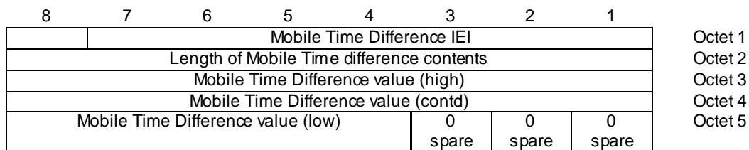
Figure 10.5.50/GSM 04.18 Mobile Time Difference information element
