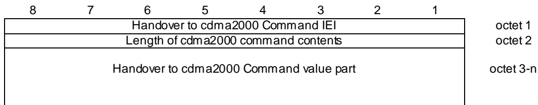
Figure 10.5.2.52/GSM 04.18: Handover to cdma2000 Command information element
