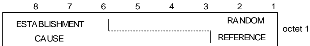
Figure 9.1/GSM 04.18: CHANNEL REQUEST message content
