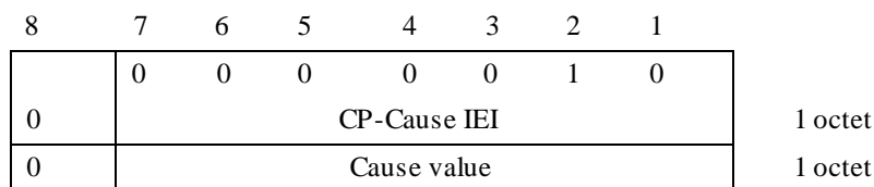
Figure 8.3/3GPP TS 04.11: CP-Cause element layout
