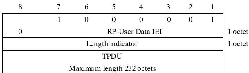
Figure 8.7/3GPP TS 04.11: RP-User data element layout
