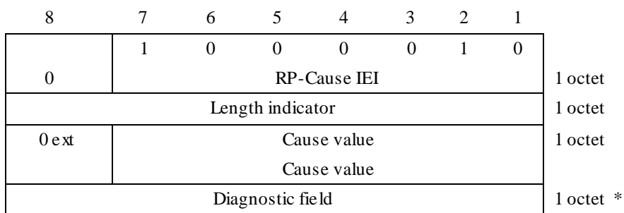
Figure 8.8/3GPP TS 04.11: RP-Cause element layout
