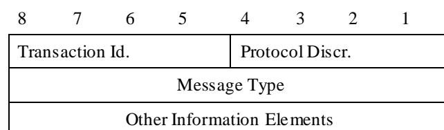
Figure 8.1/3GPP TS 04.11
