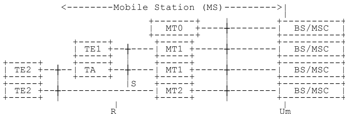
Figure 1: GSM PLMN Access Reference Configuration
