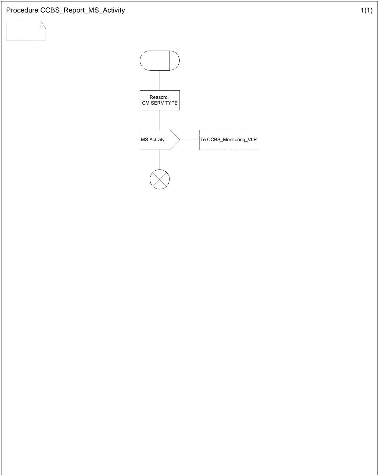
Figure 11.3.6: Procedure CCBS_Report_MS_Activity
