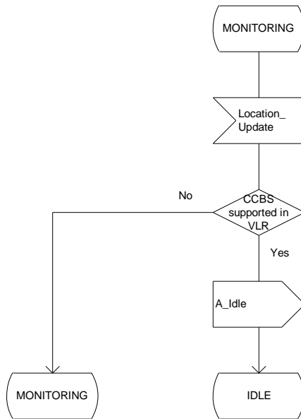
Figure 11.1.2.6: Process HLRA_Monitoring (sheet 2 of 2)
