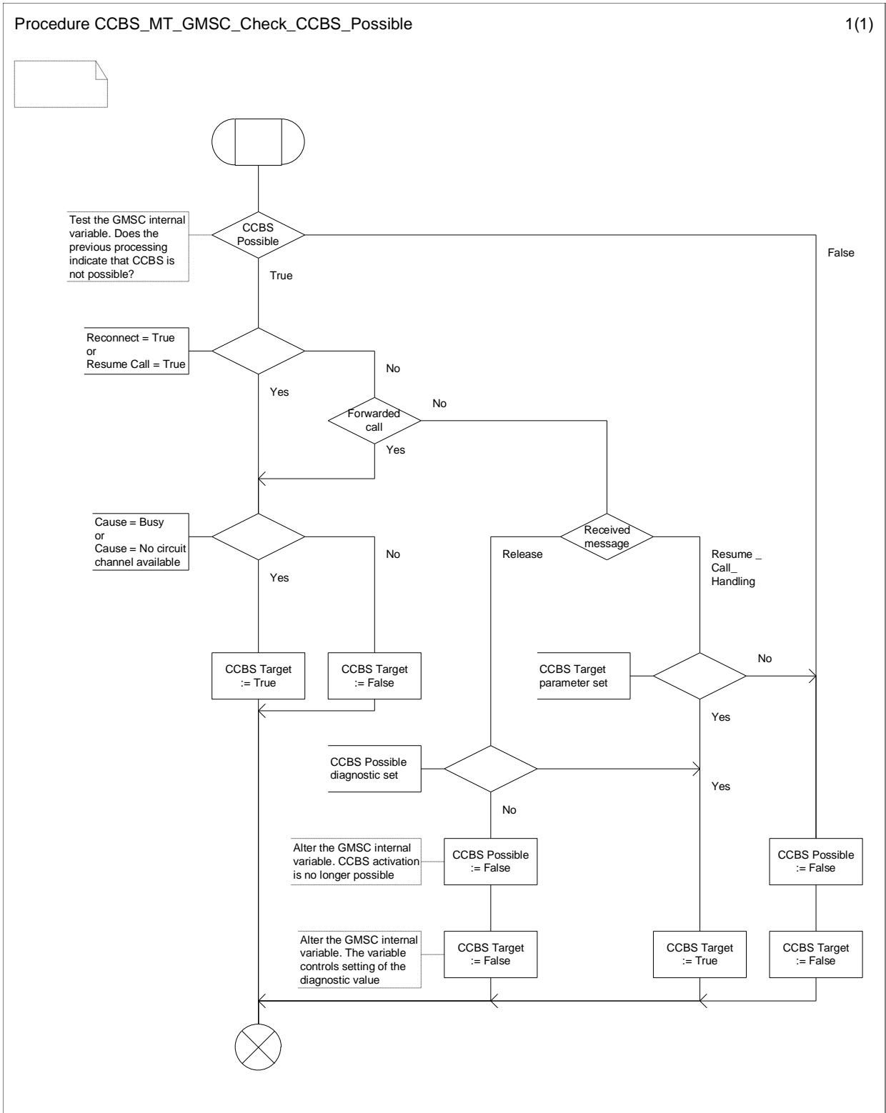
Figure 11.2.1.5: Procedure CCBS_MT_GMSC_Check_CCBS_Possible
