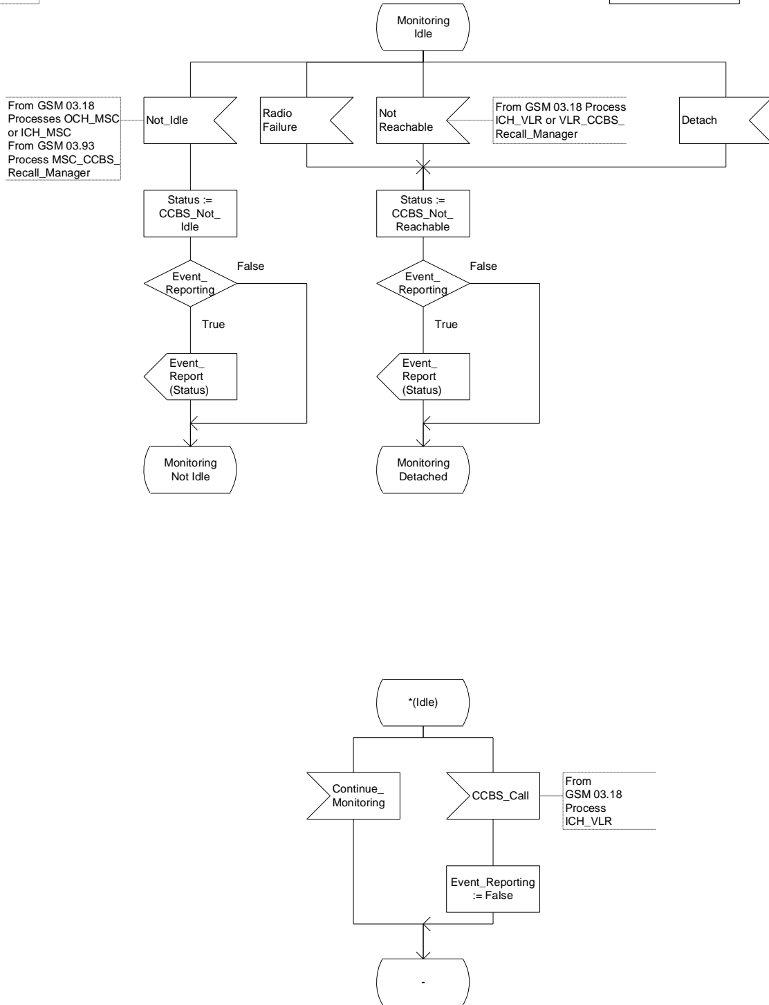
Figure 11.3.1: Process CCBS_Monitoring_VLR (sheet 3 of 4)
