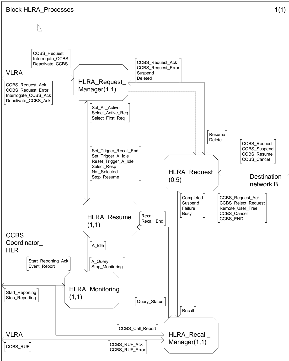
Figure 11.1.2.1: HLRA Processes
