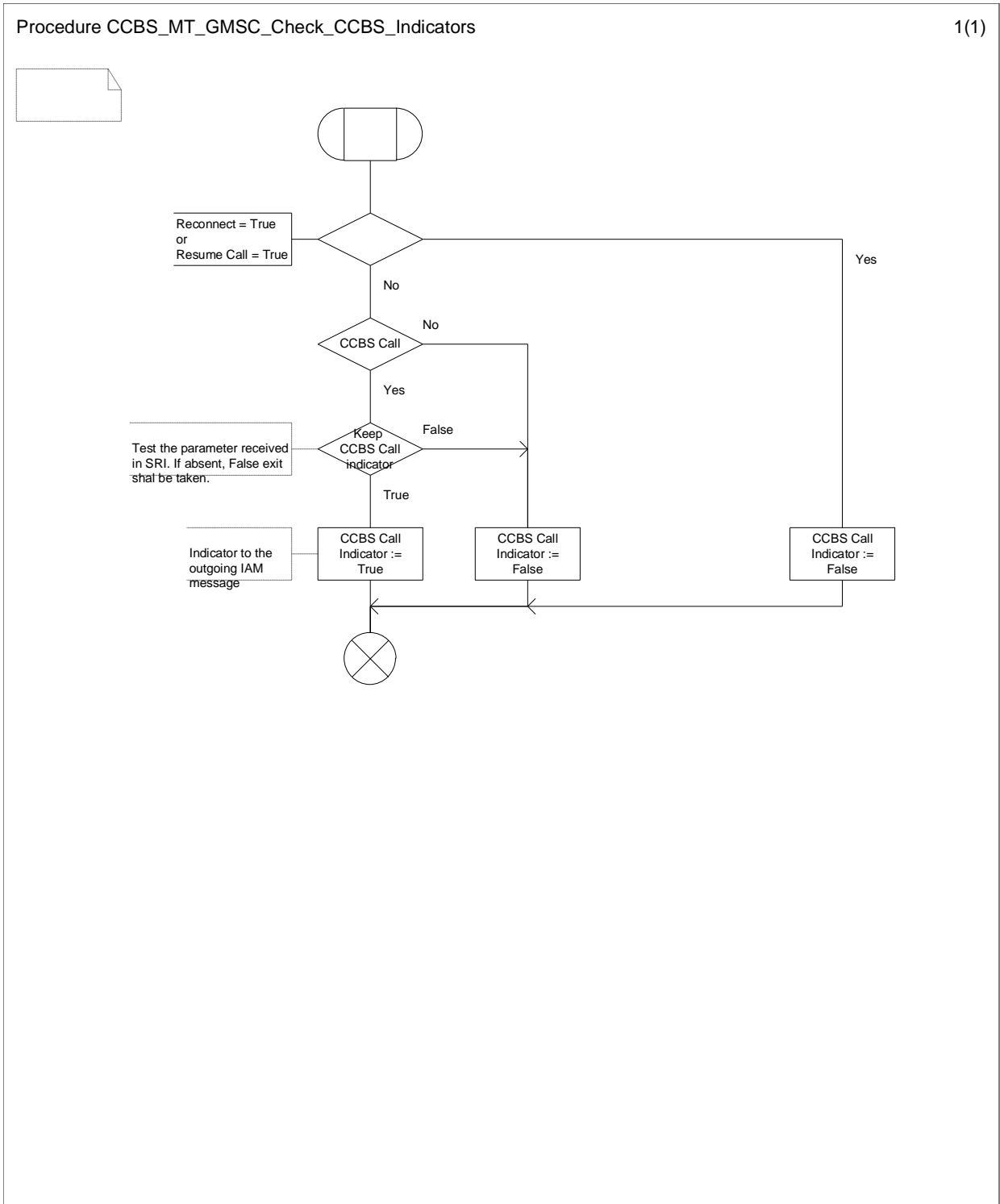
Figure 11.2.1.2: Procedure CCBS_MT_GMSC_Check_CCBS_Indicators
