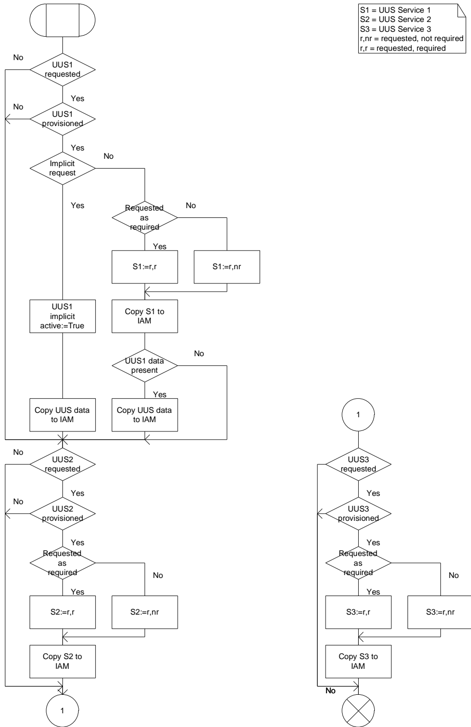
Figure 9.1.1.2: Procedure UUS_OCH_Set_Info_In_IAM
