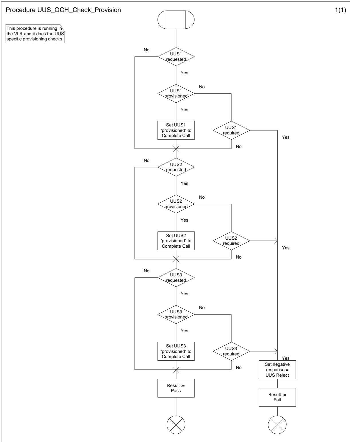
Figure 9.1.2.1: Procedure UUS_OCH_Check_Provision
