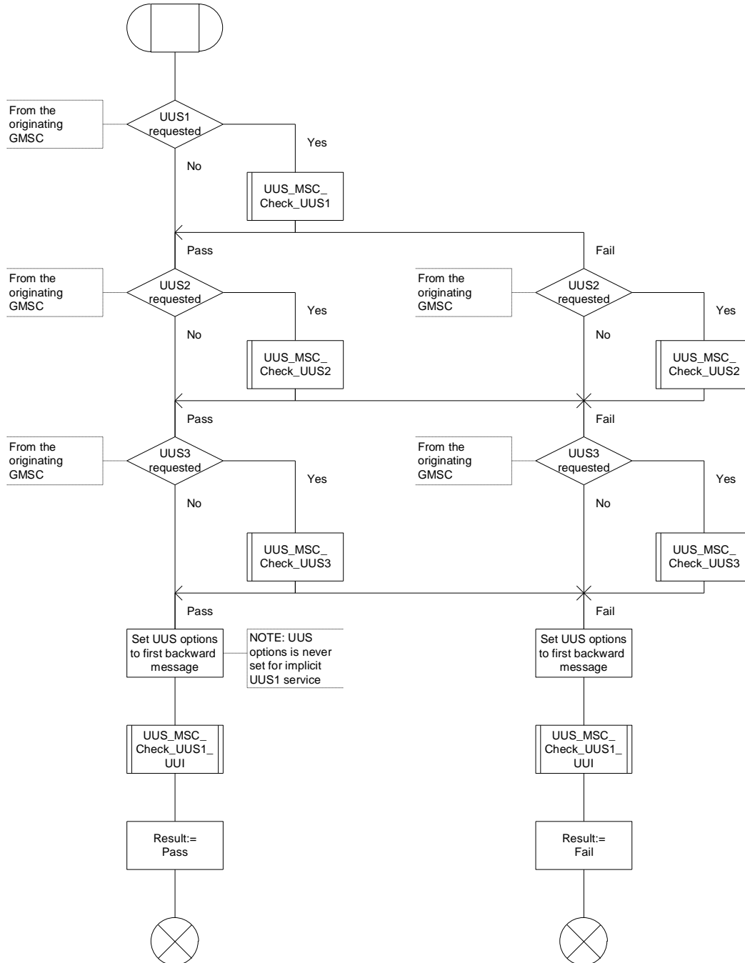
Figure 9.2.2.1: Procedure UUS_ICH_Check_Support
