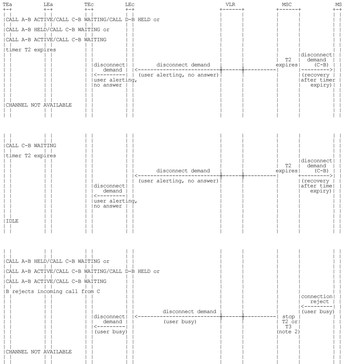
Figure 1.6 (sheet 2 of 7): Information flow for call waiting
