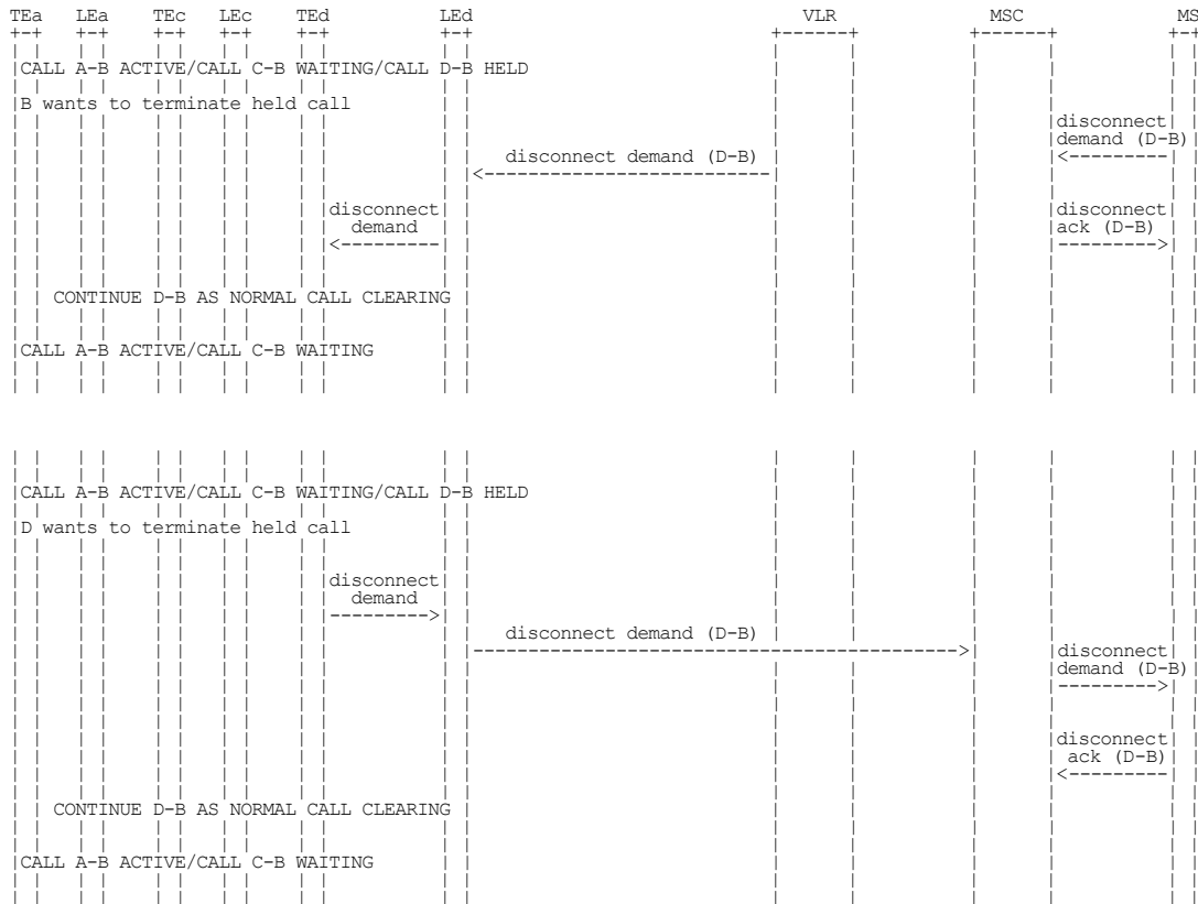
Figure 1.6 (sheet 7 of 7): Information flow for call waiting
