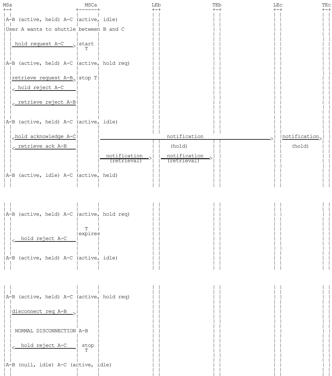
Figure 2.3 (sheet 2 of 3): Information flow for call hold
