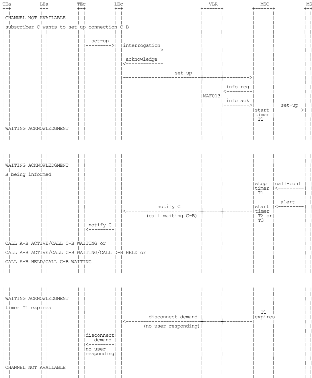
Figure 1.6 (sheet 1 of 7): Information flow for call waiting
