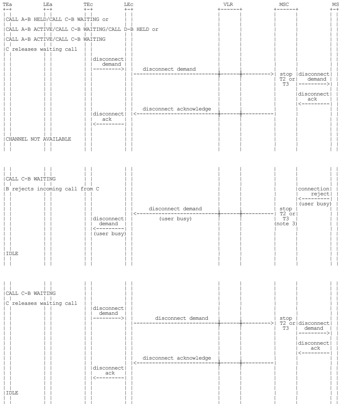
Figure 1.6 (sheet 3 of 7): Information flow for call waiting
