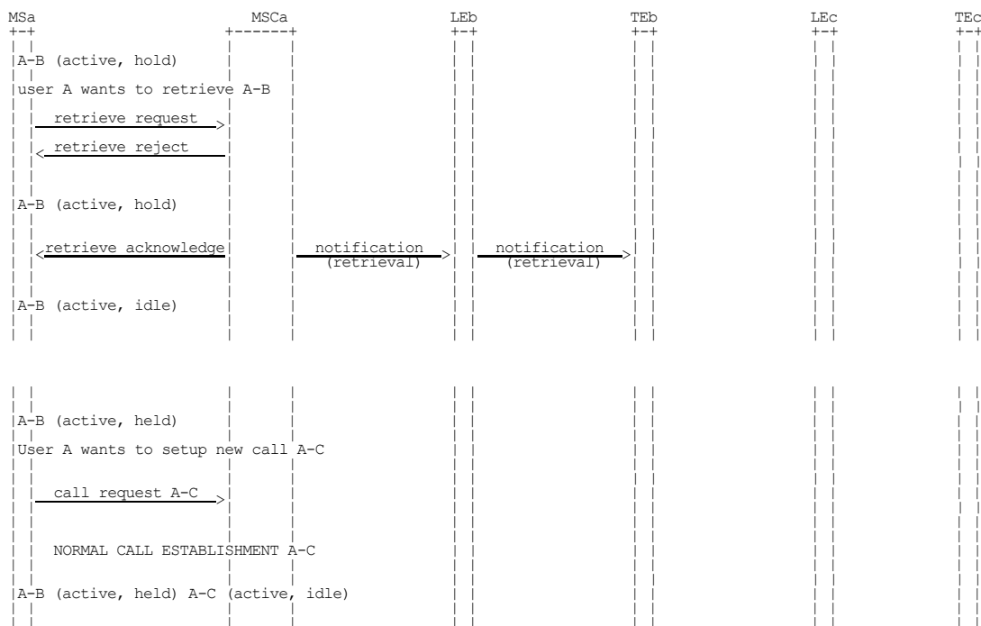
Figure 2.3 (sheet 1 of 3): Information flow for call hold
