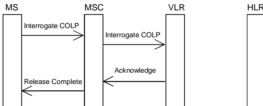
Figure 3.1: Interrogation of connected line identification presentation
