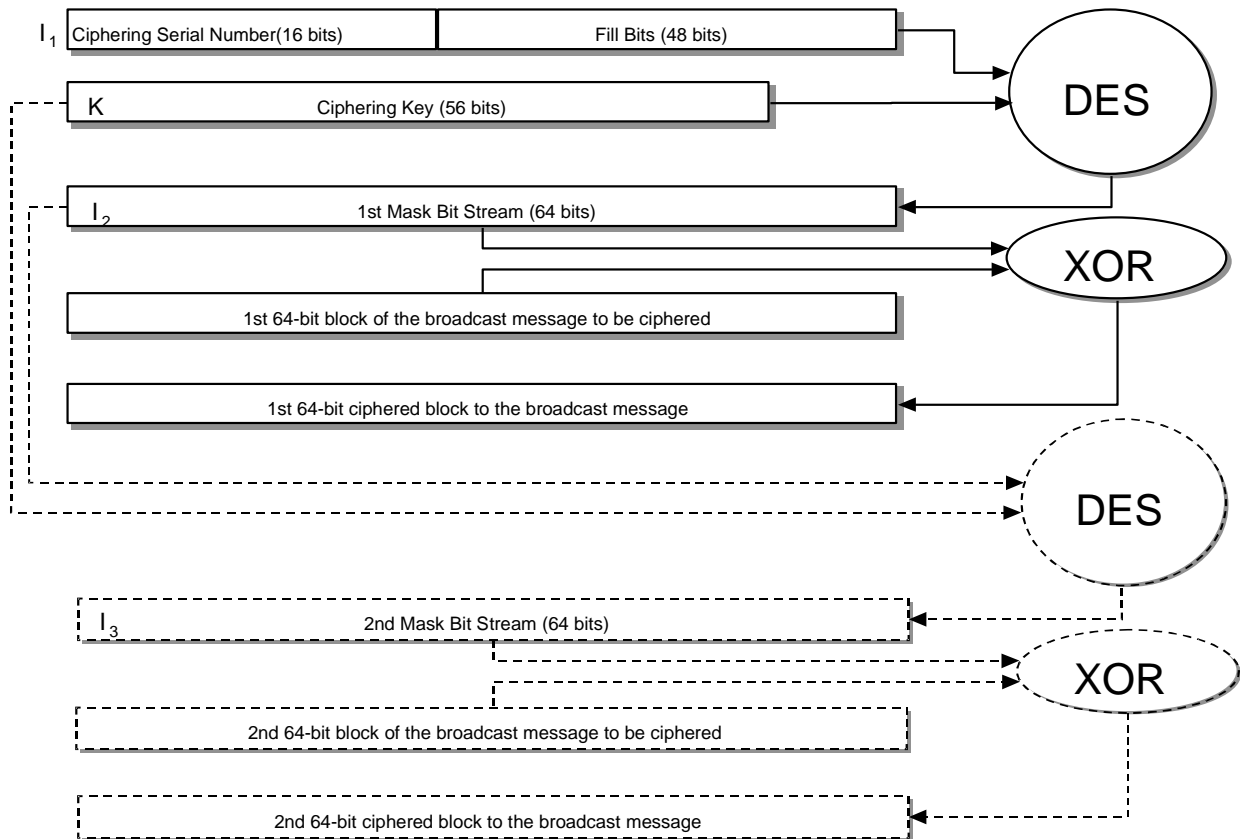
Figure 61: CIPHERING ALGORITHM
