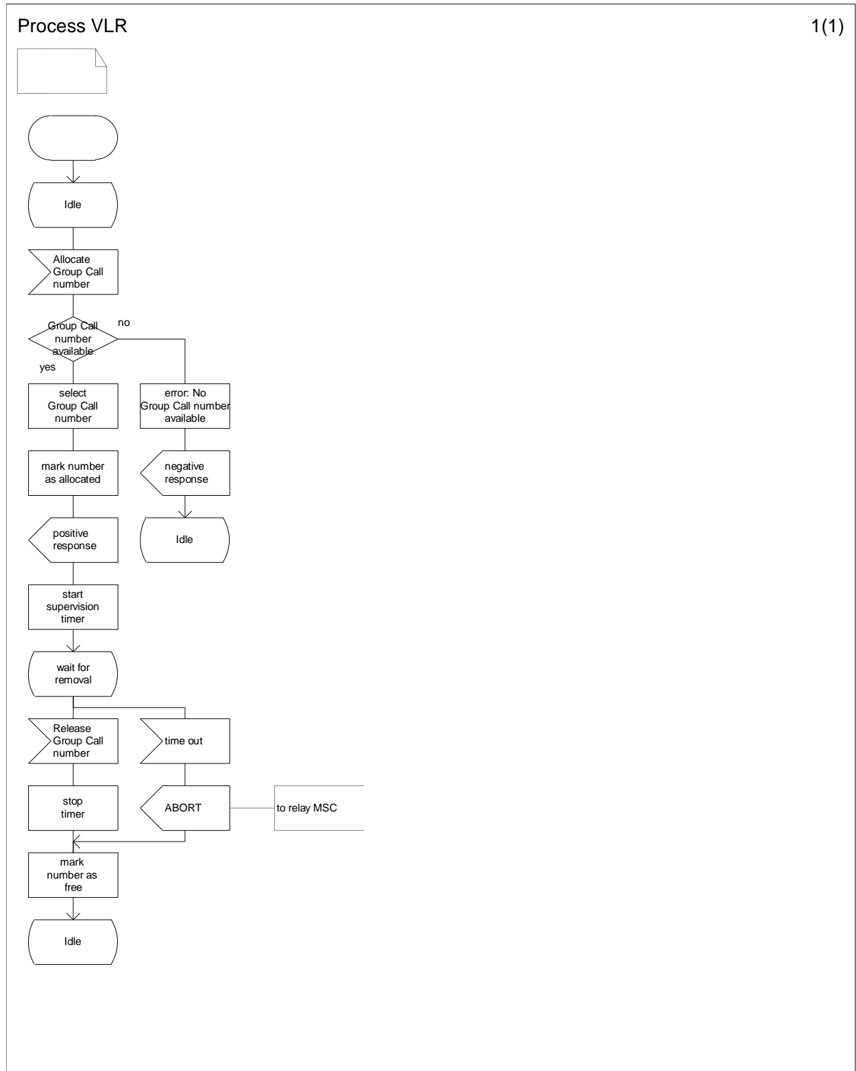
Figure 9: Group Call number allocation process in the VLR
