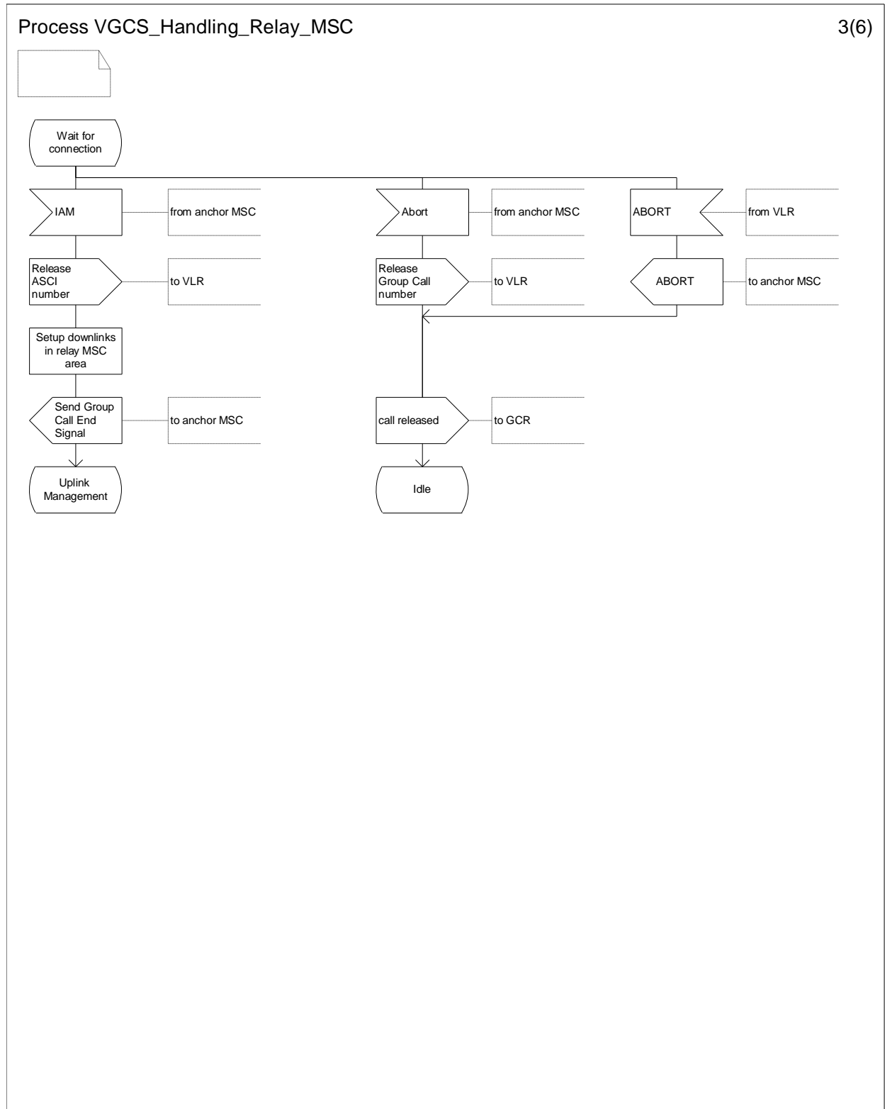
Figure 10: The VGCS handling process in the relay MSC (sheet 3 of 6)
