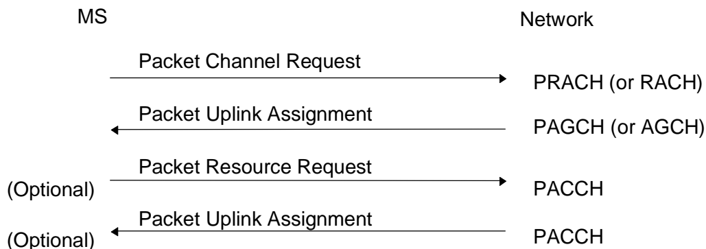
Figure 23: Access and allocation for the one or two phase packet access, uplink packet transfer
