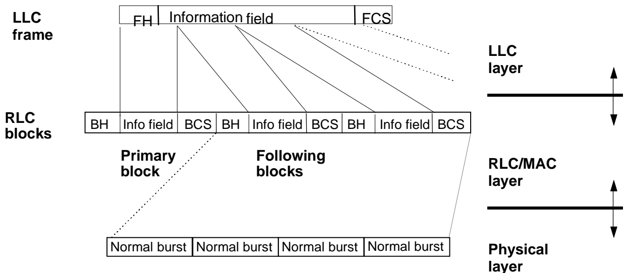
Figure 21: Transmission and reception data flow for EGPRS MCS-7
