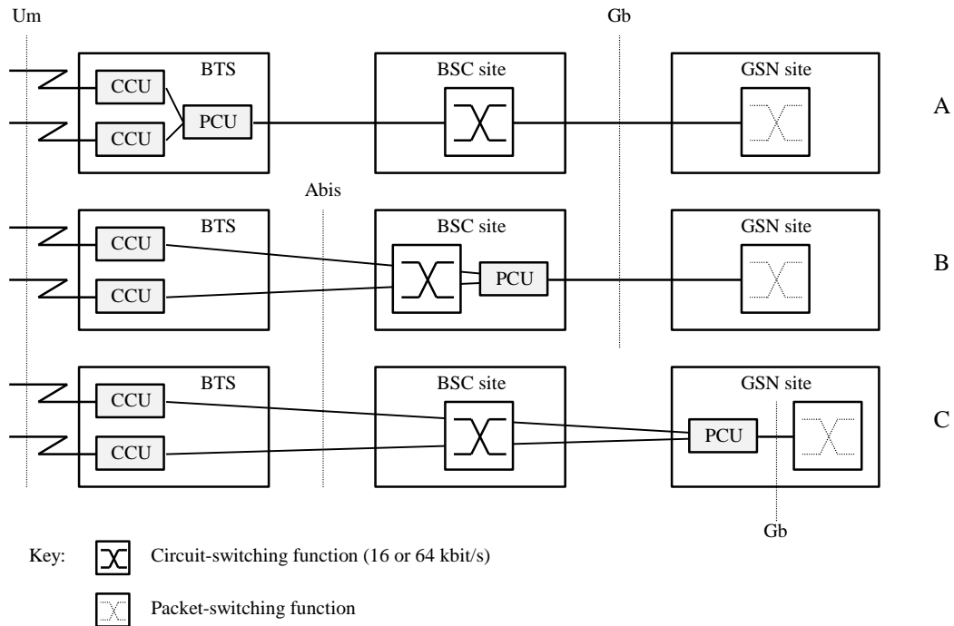
Figure 50: Remote Packet Control Unit (PCU) Positions
