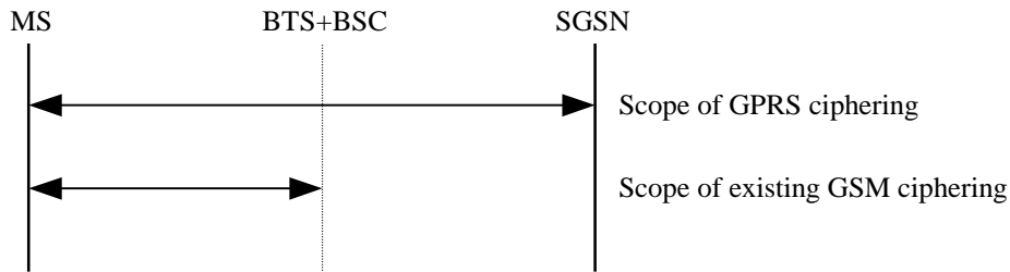
Figure 25: Scope of GPRS Cipherng
