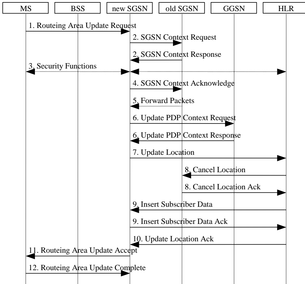
Figure 28: Inter SGSN Routing Area Update Procedure
