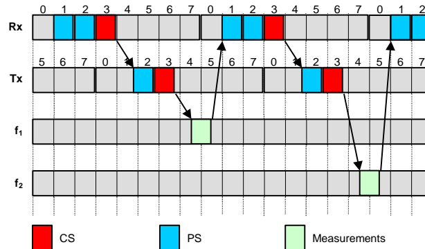
Figure 1: Example of multislots configuration of a GPRS simple class A mobile station in dual transfer mode.
