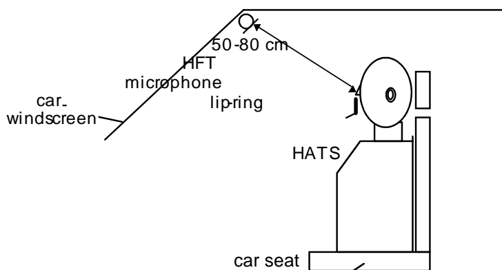
Figure 10: Measurement configuration for car type applications
