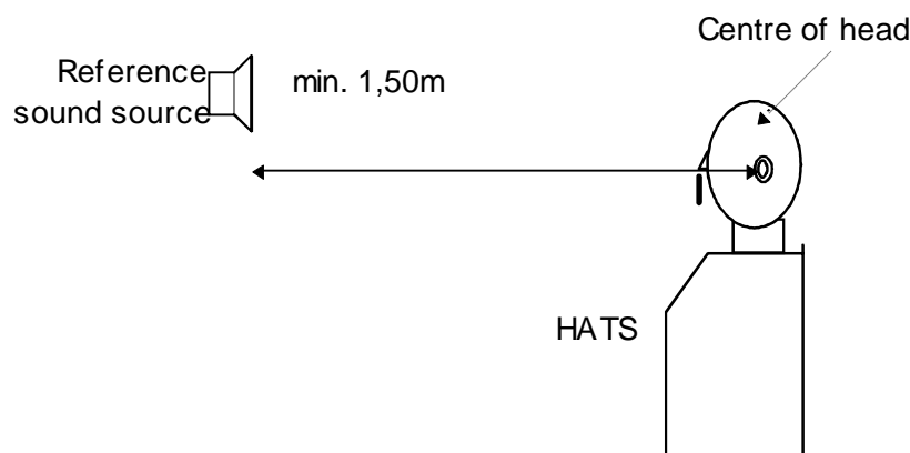
Figure 11: Set-up for HATS free field calibration in an anechoic chamber
