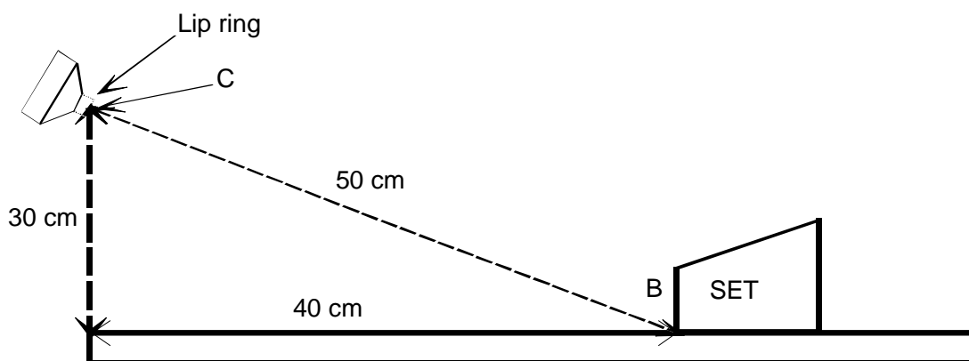
Figure 9: Measurement configuration
