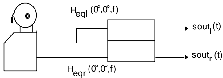
Figure 12: Measurement set-up for HATS ( H_{eq_l}(0^\circ, 0^\circ, f) = free-field equalizer left ear, H_{eq_r}(0^\circ, 0^\circ, f) = free-field equalizer right ear)
