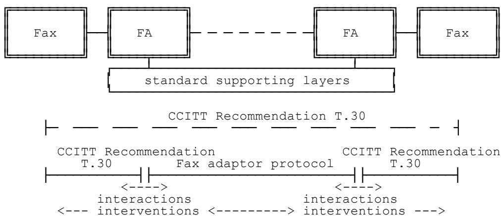
Figure 6/03.46: Communication model
