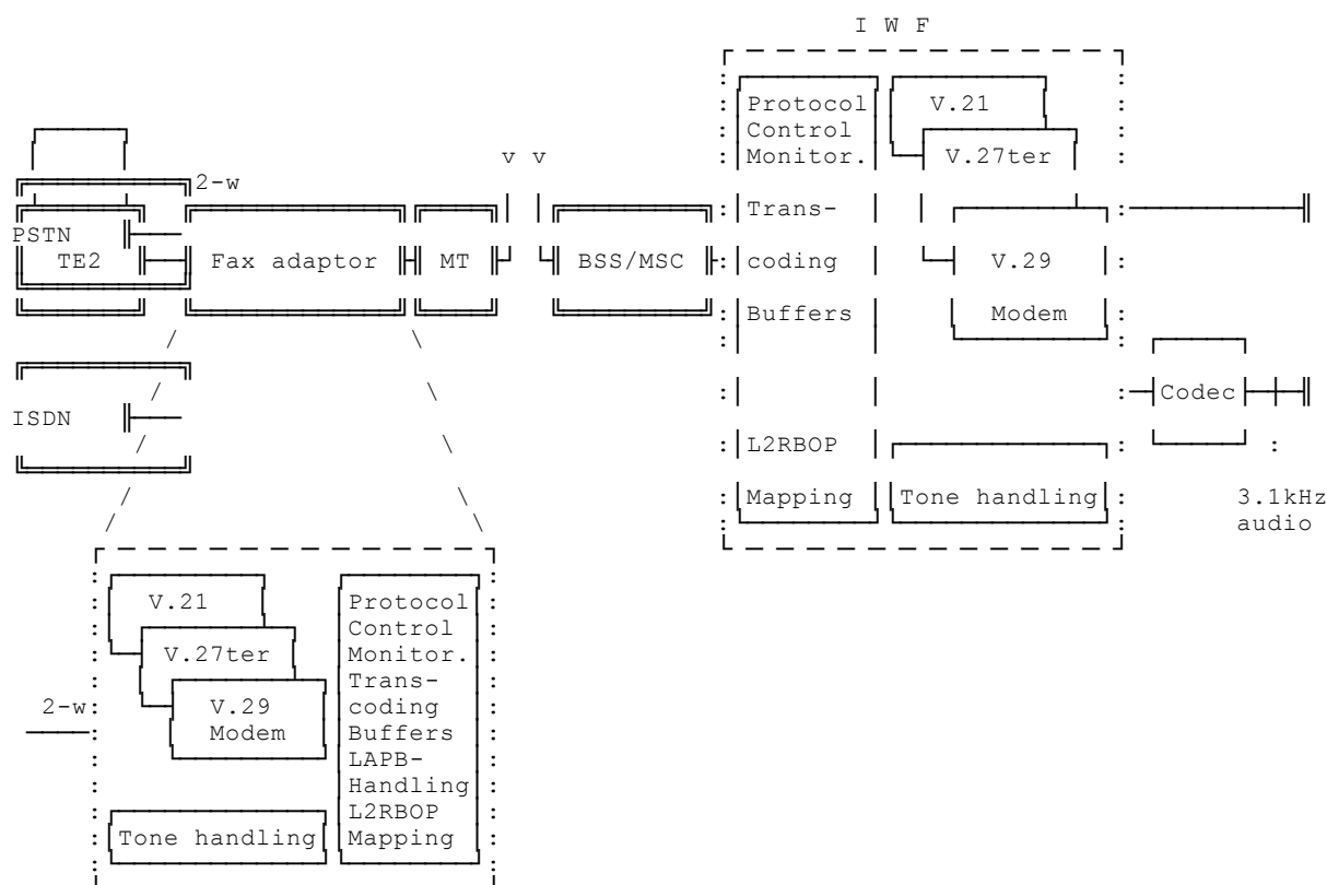
Figure 7/03.46: Network interworking
