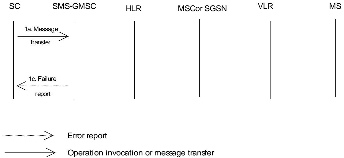
Figure 03.40/15b): Short message transfer attempt failing due to error at the SMS-GMSC
