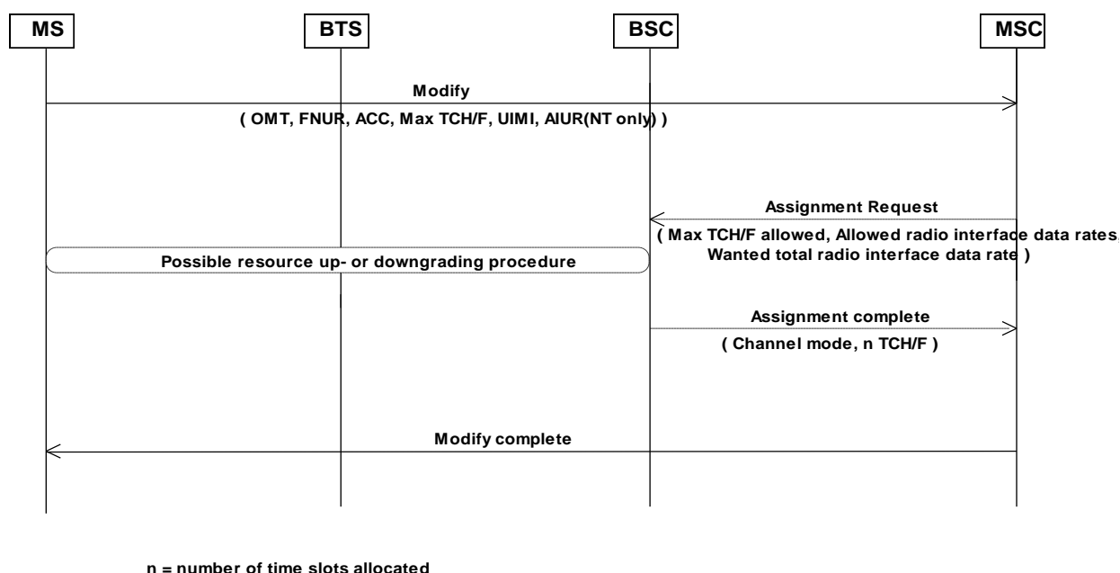
Figure 9: User initiated service level up- and downgrading
