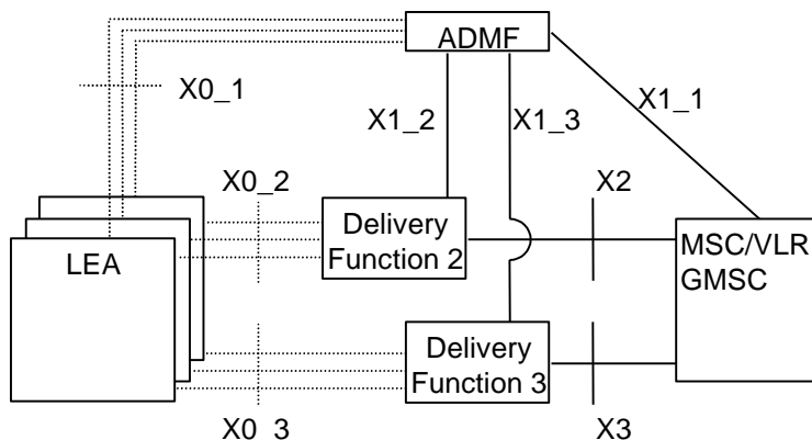
Figure 1: Reference configuration
