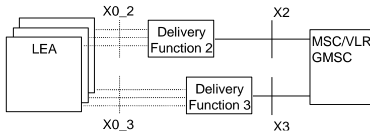
Figure 11: Functional model for Lawful Interception invocation
