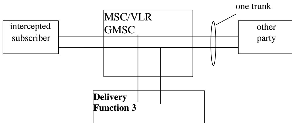
Figure 12: Bridged Access
