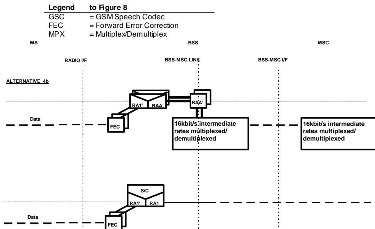
Figure 8 (concluded): Location of transcoding and rate adaptation
