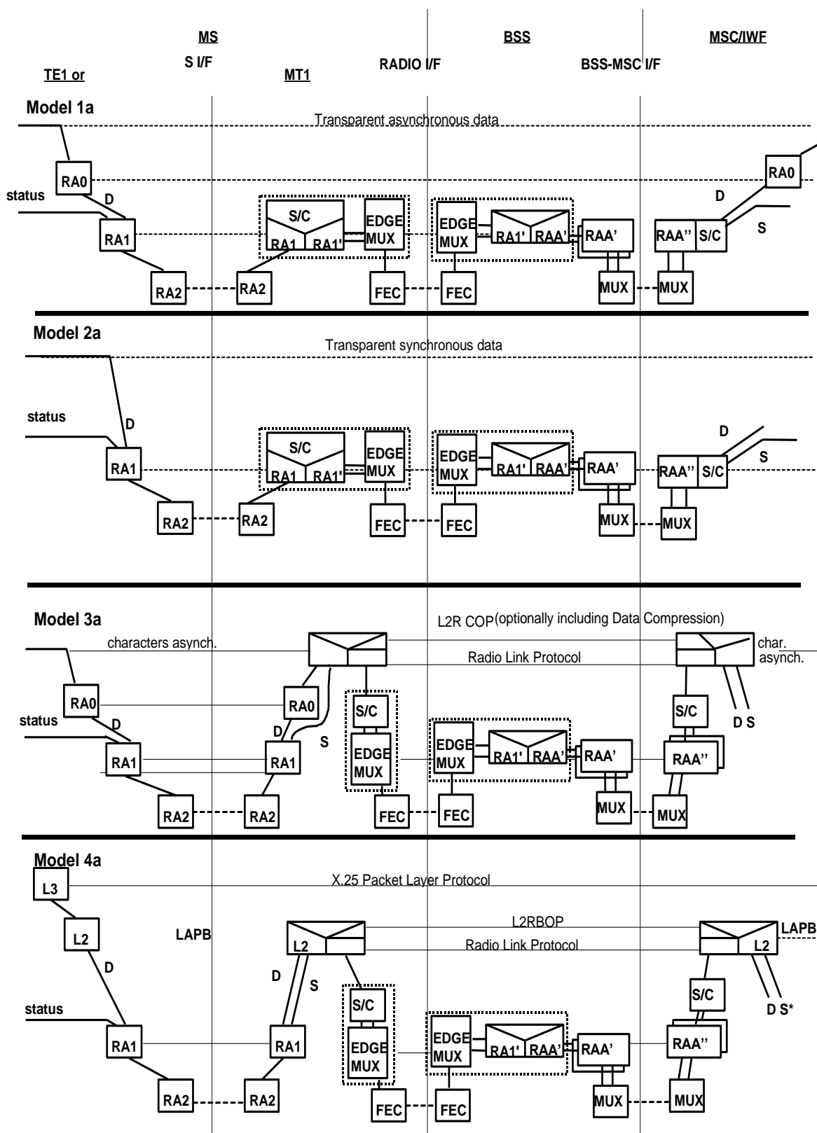
Figure 8 : Information transfer protocol models for GSM PLMN connections using EDGE channels
