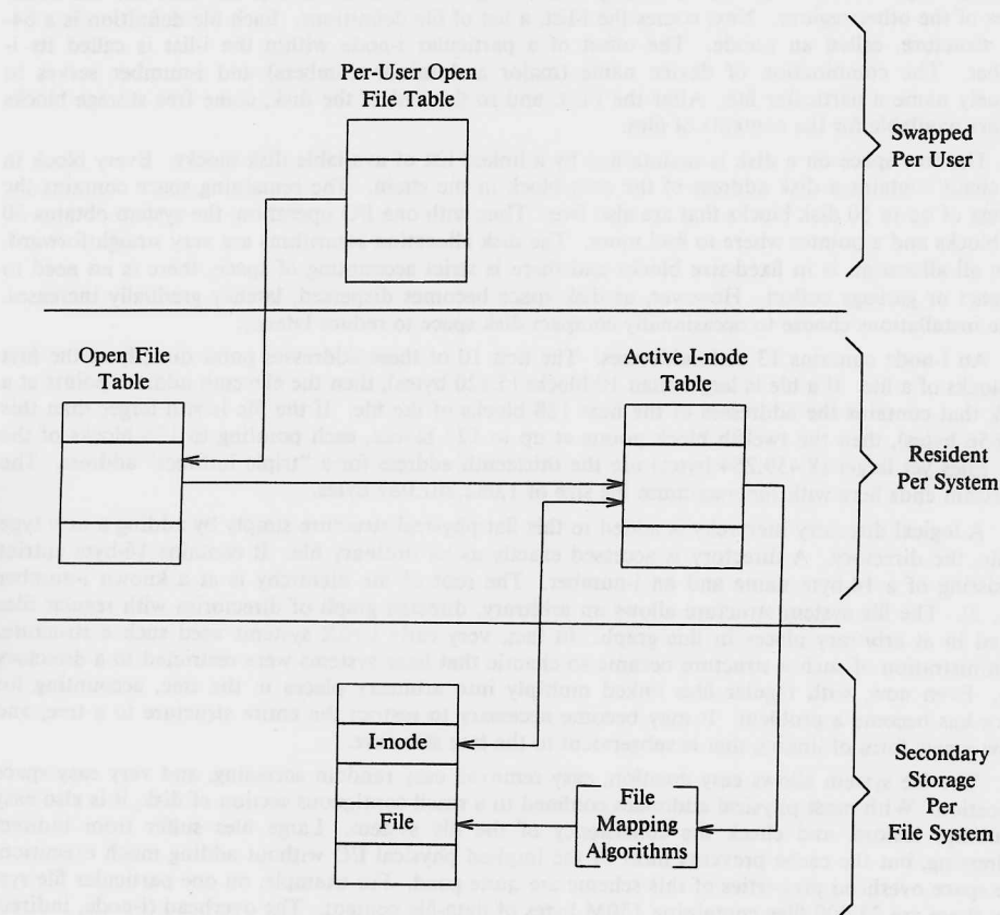
Fig. 2—File system data structure.
