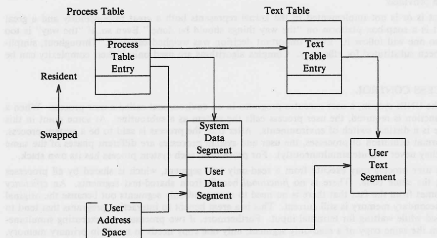
Fig. 1—Process control data structure.
