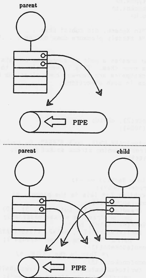
Figure 2 Sharing a pipe between parent and child
